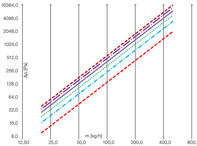
KORALINE LD 30/26
